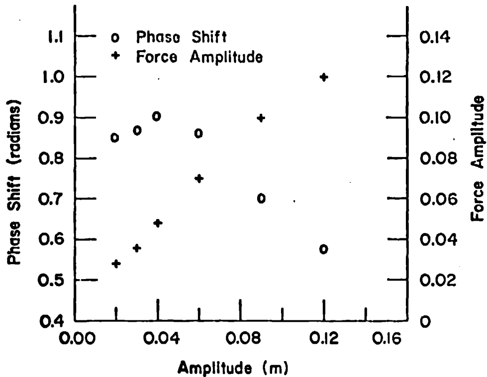
Fig. 1. Phase shift and amplitude of the dynamic pressure force as functions of the wedge displacement amplitude.
